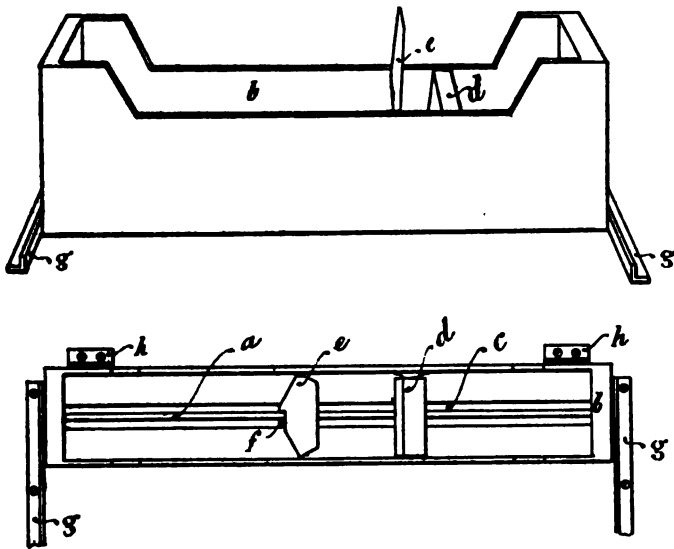
FIG. 89.—Elevation and Plan of Card-Charging Tray (Section 298).
